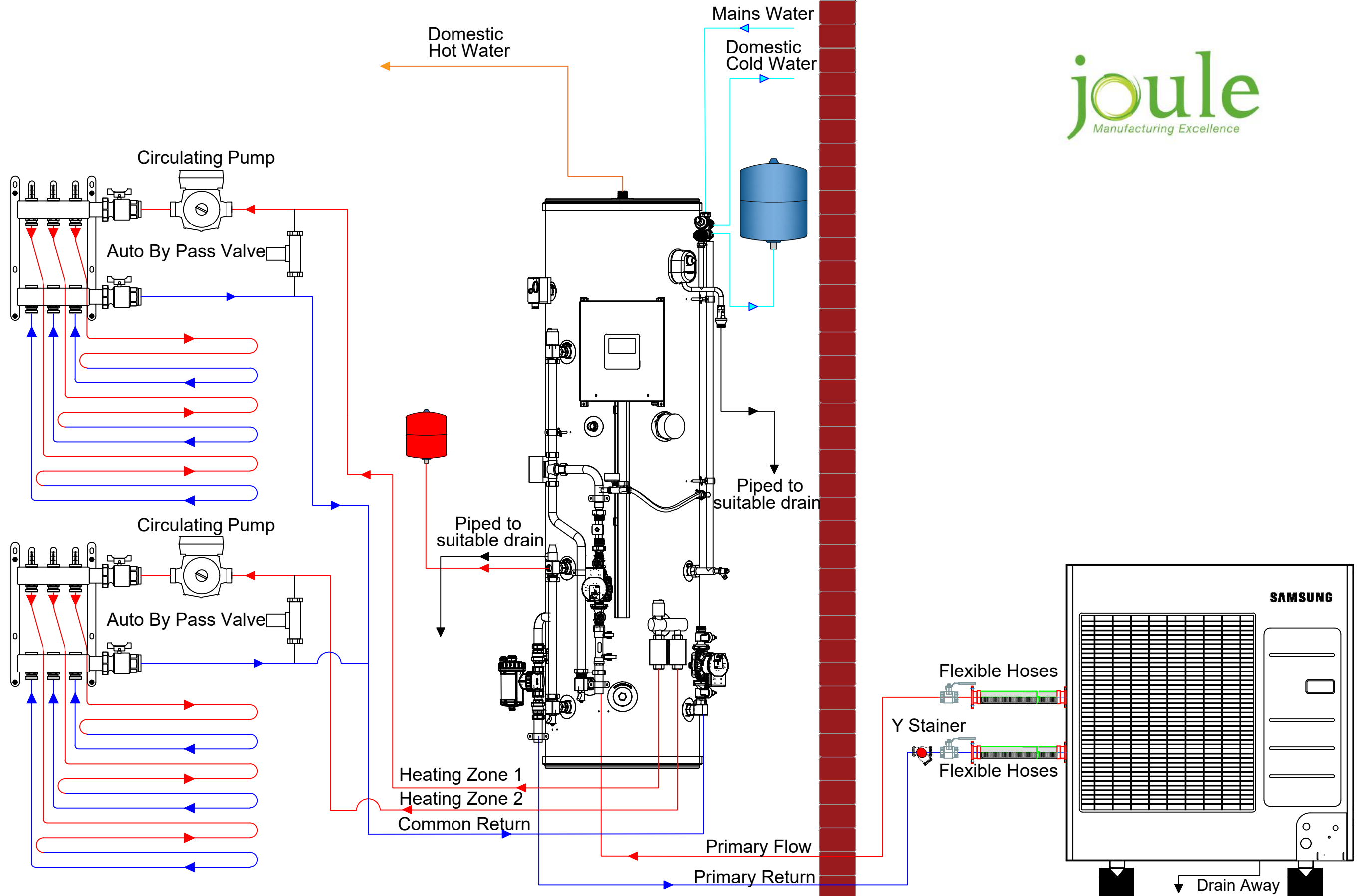
SAMSUNG ASHP WITH ZENITH DHW AND 2 HEATING ZONE 2 x UFHs
