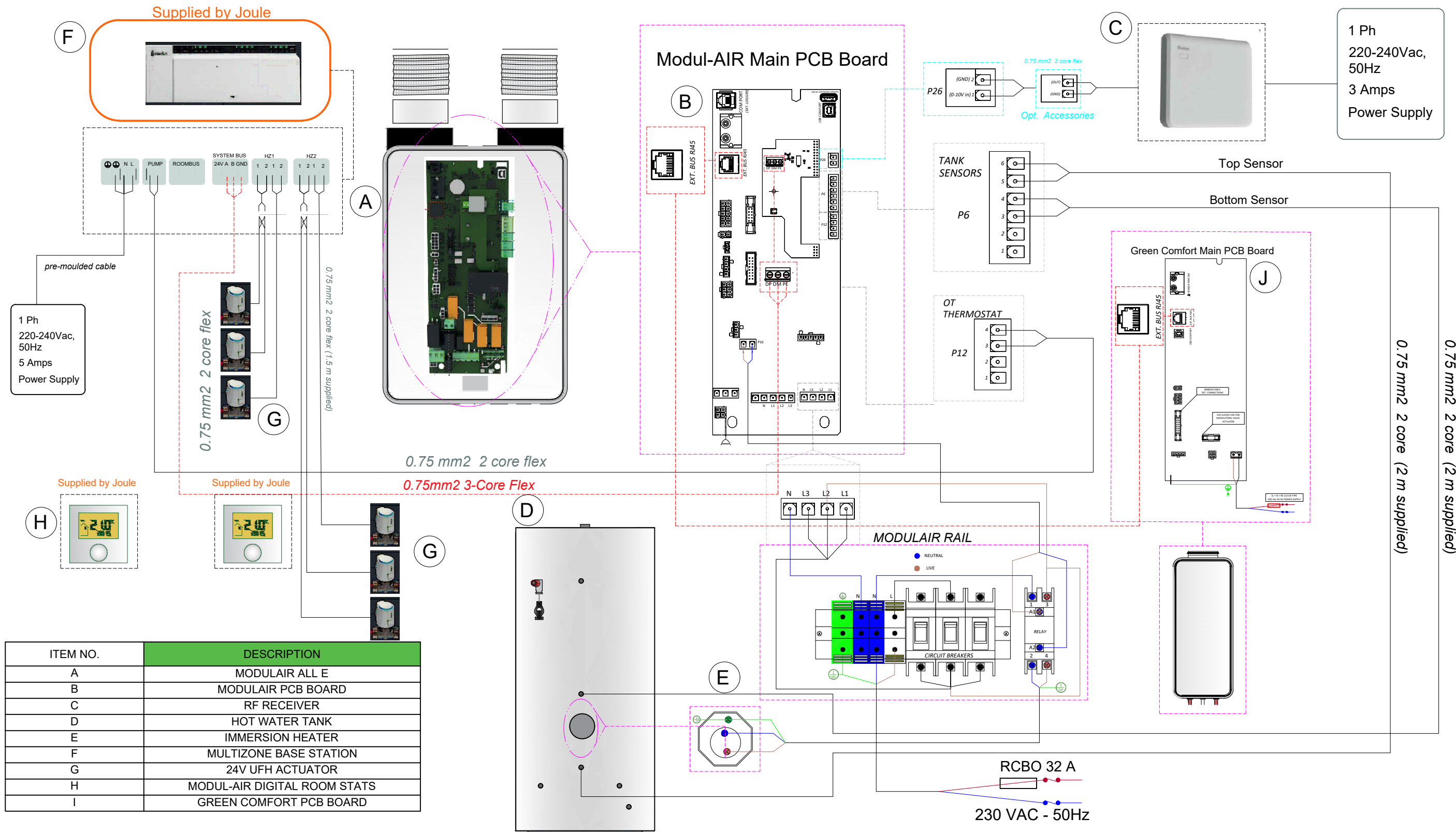
Modulaire All-E & GC with 2 Zone UFH Electrical Schematic
