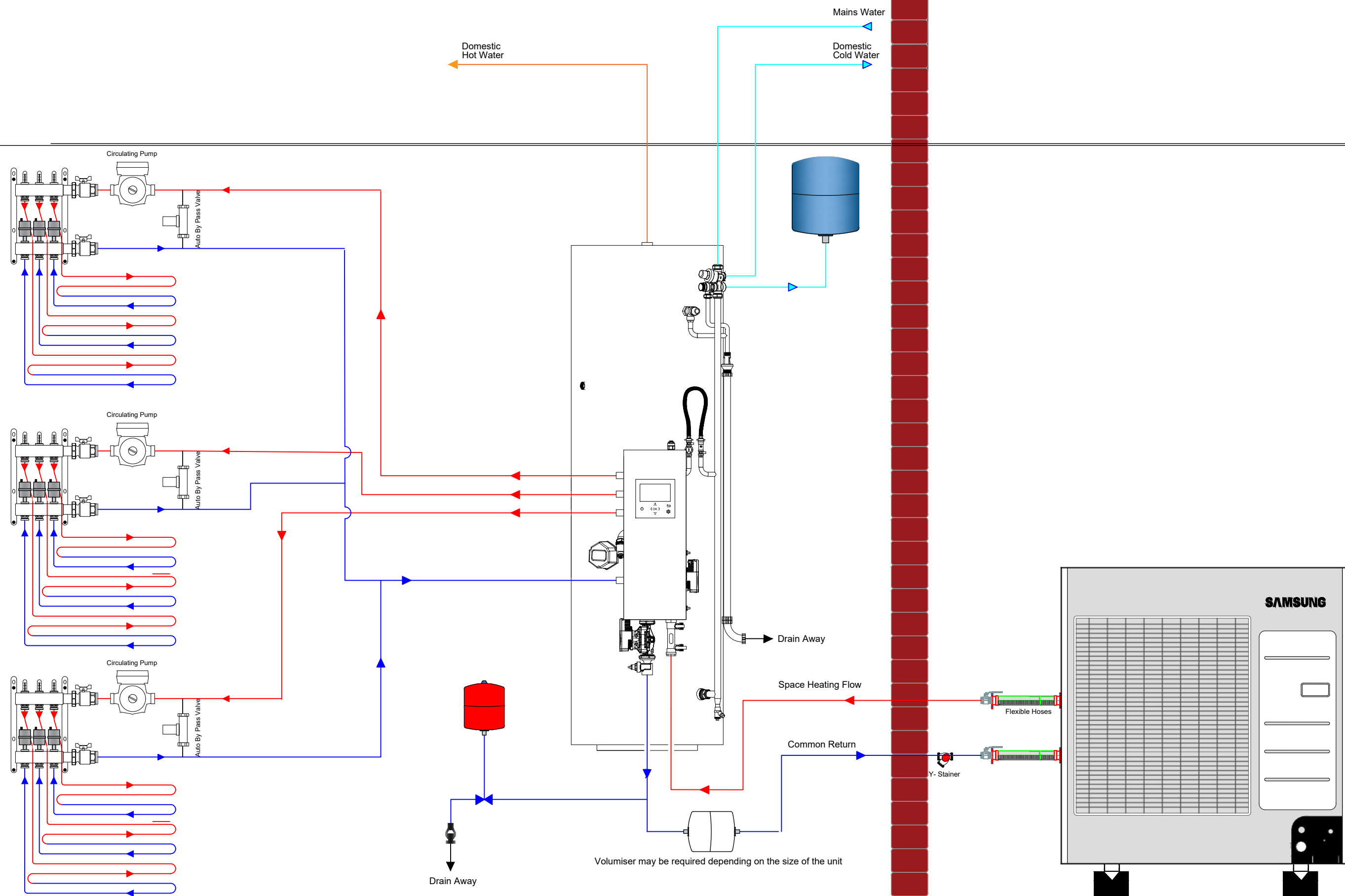
SAMSUNG ASHP WITH KODIAK DHW WITH 3 HEATING ZONE 3 x UFH
