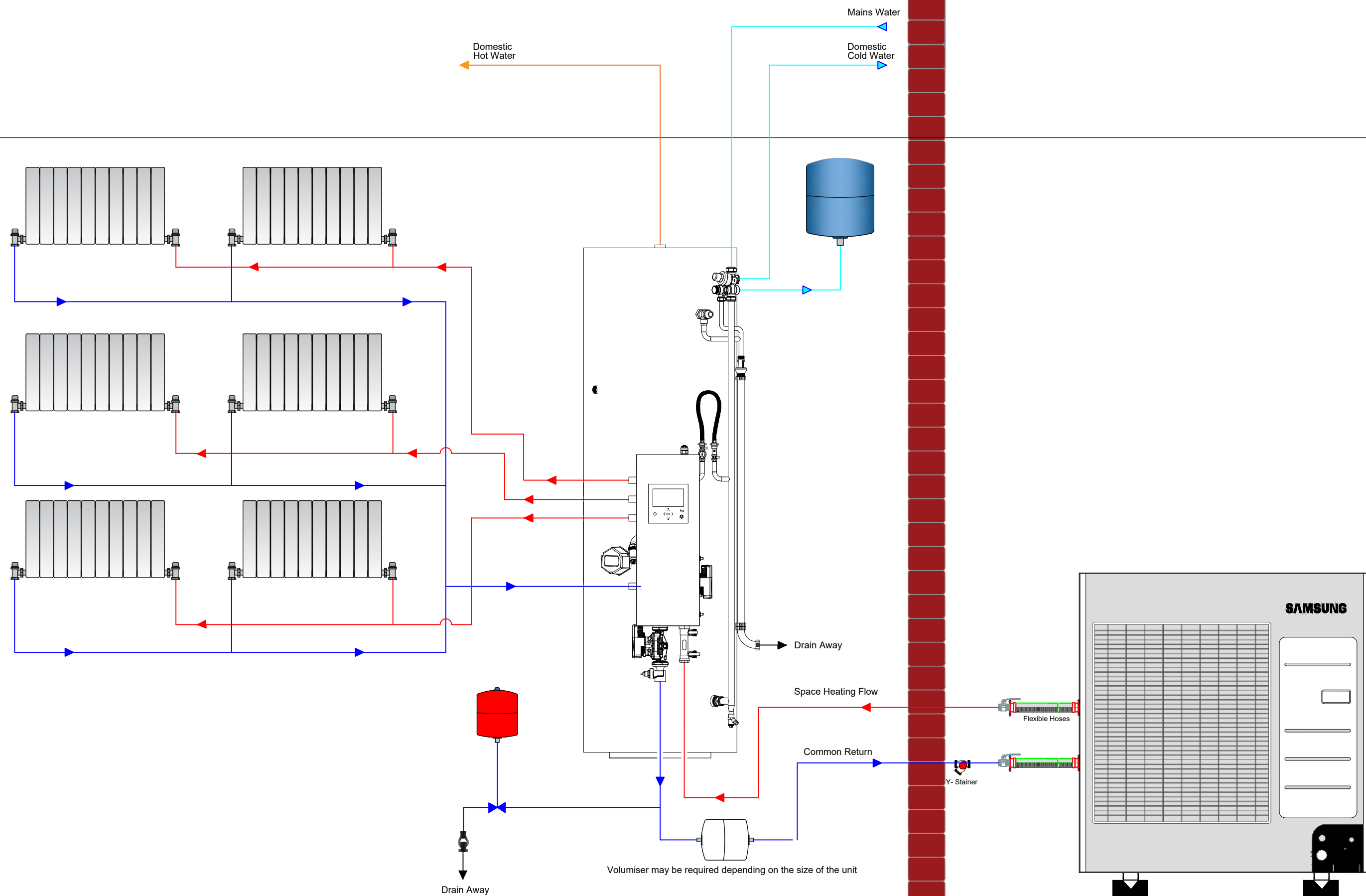
SAMSUNG ASHP WITH KODIAK DHW WITH 3 HEATING ZONE 3 RAD
