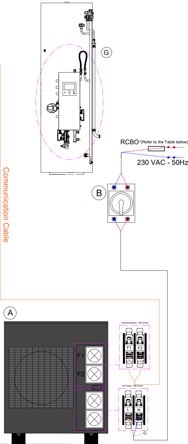
Front View of Unit & Cylinder
