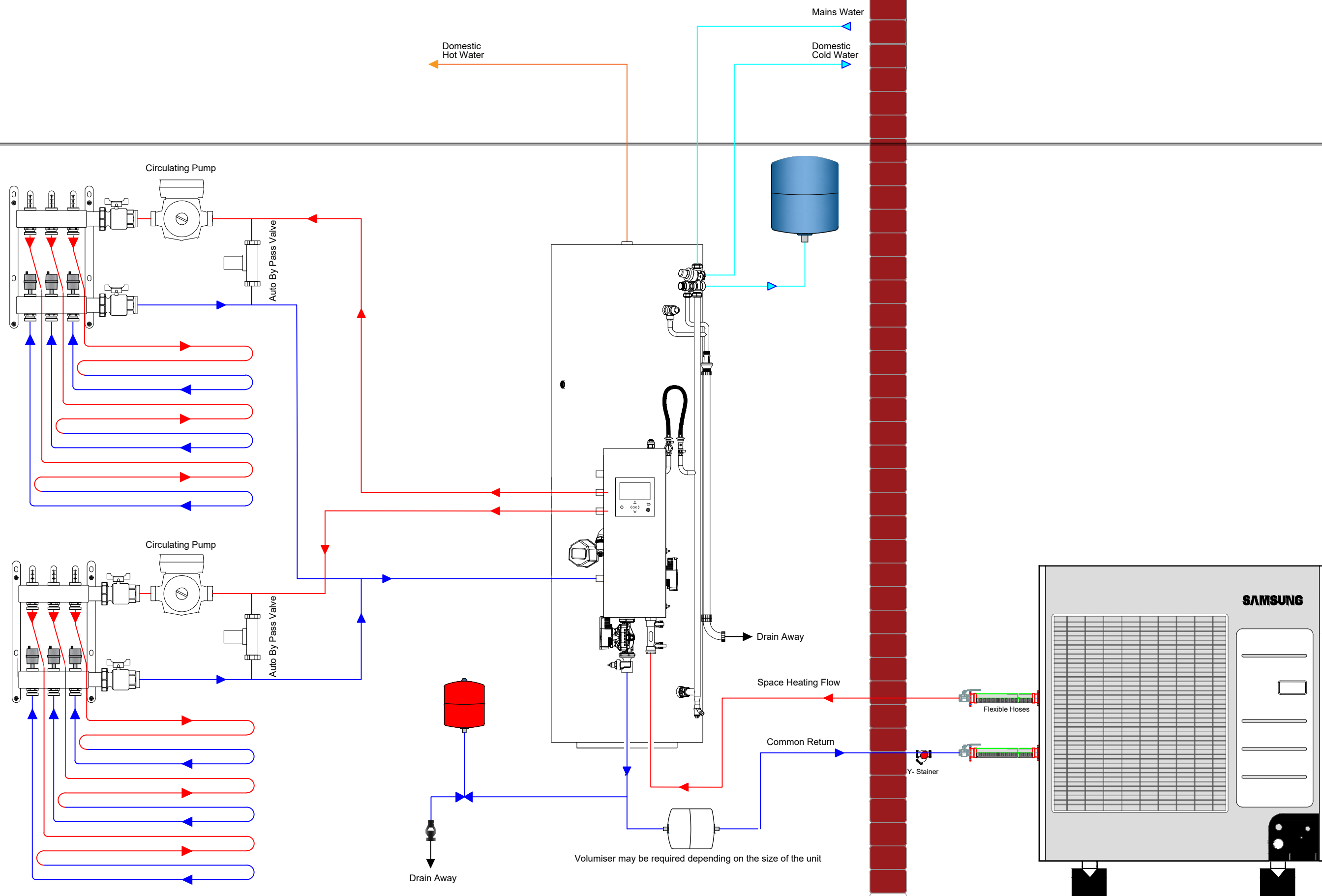
SAMSUNG ASHP WITH KODIAK DHW WITH 2 HEATING ZONE 2 x UFH
