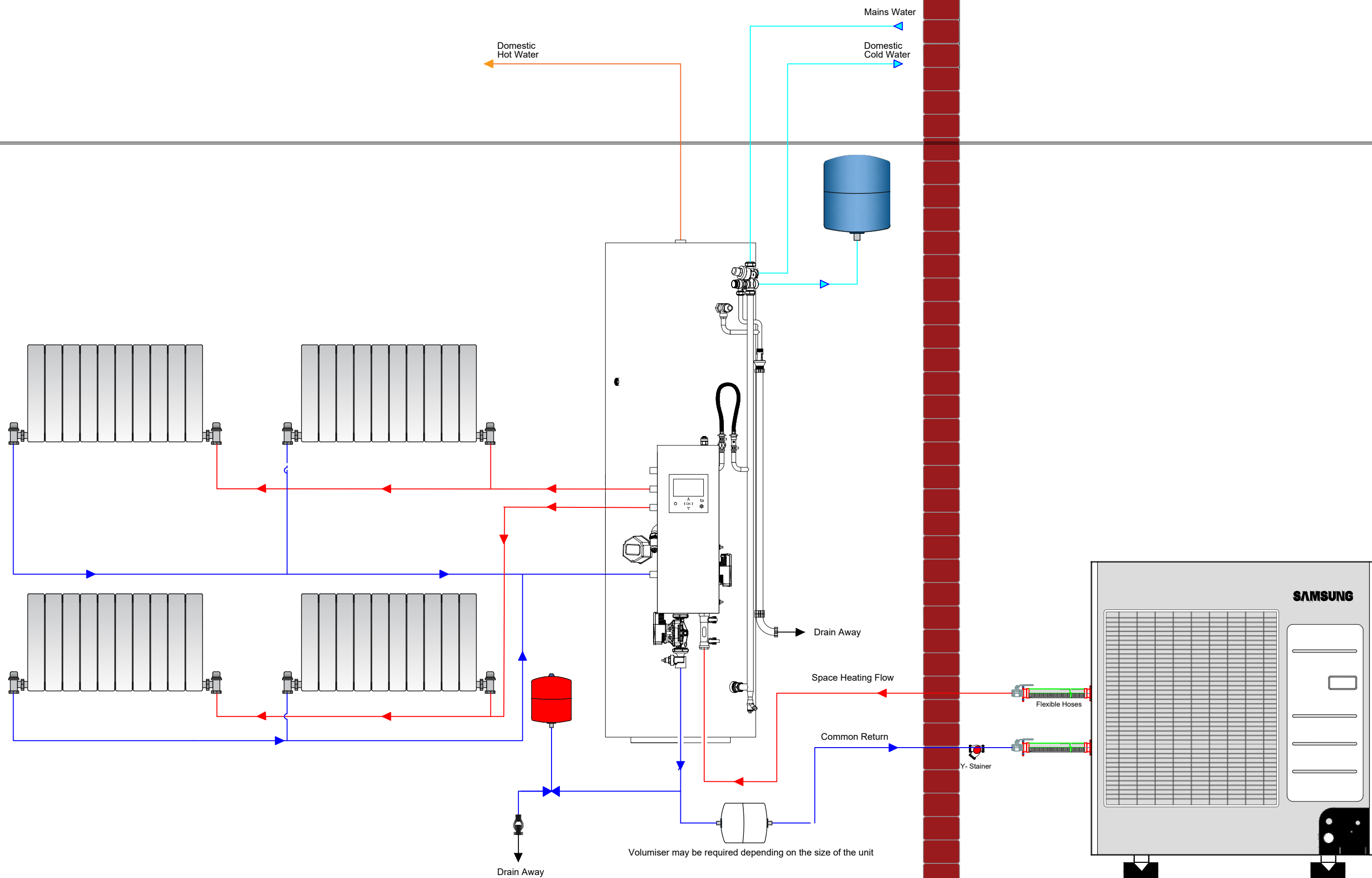
SAMSUNG ASHP WITH KODIAK DHW WITH 2 HEATING ZONE 2 x RADS
