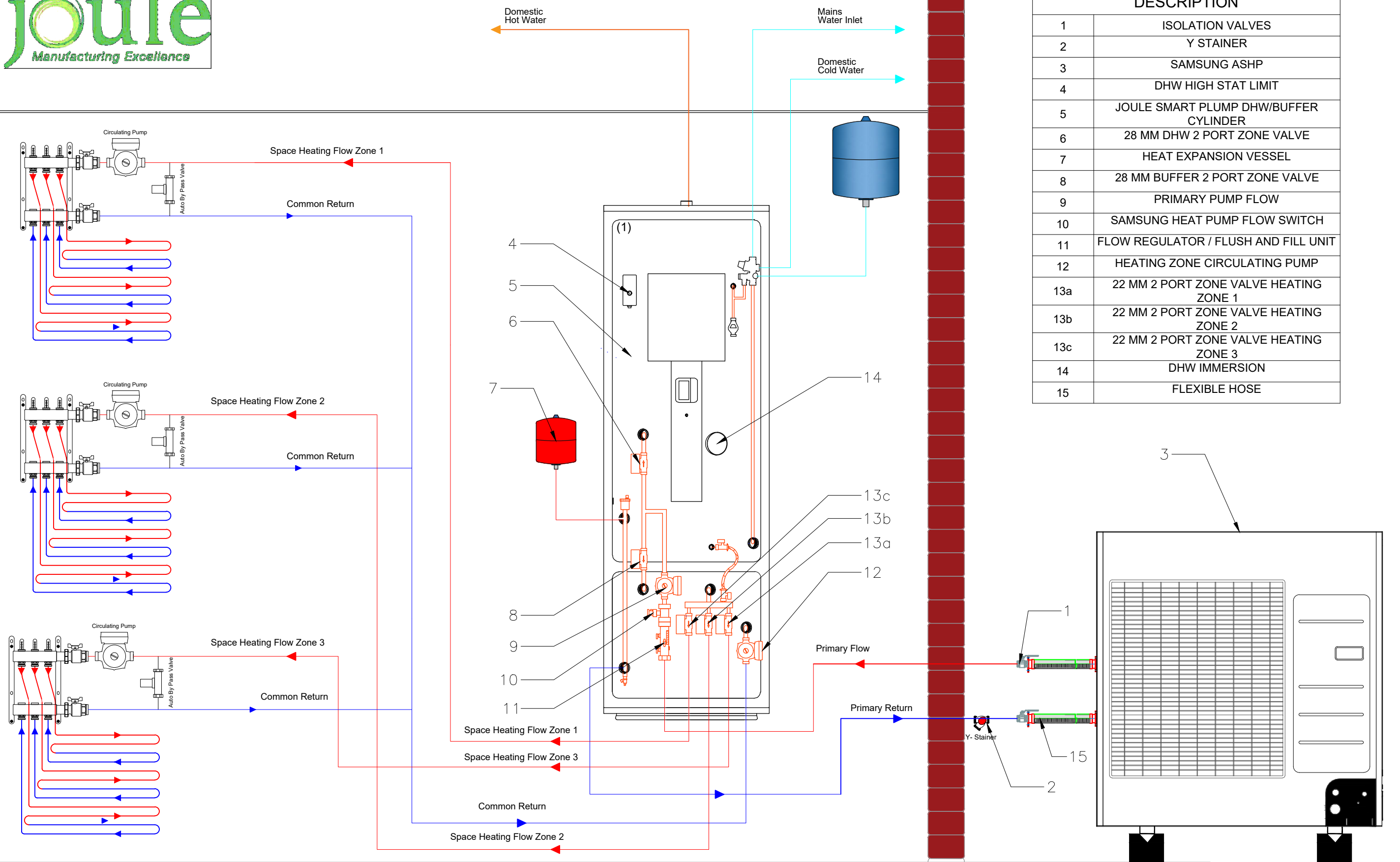
SAMSUNG ASHP WITH SMARTPLUMB DHW WITH 3 HEATING ZONE 3XUFHs
