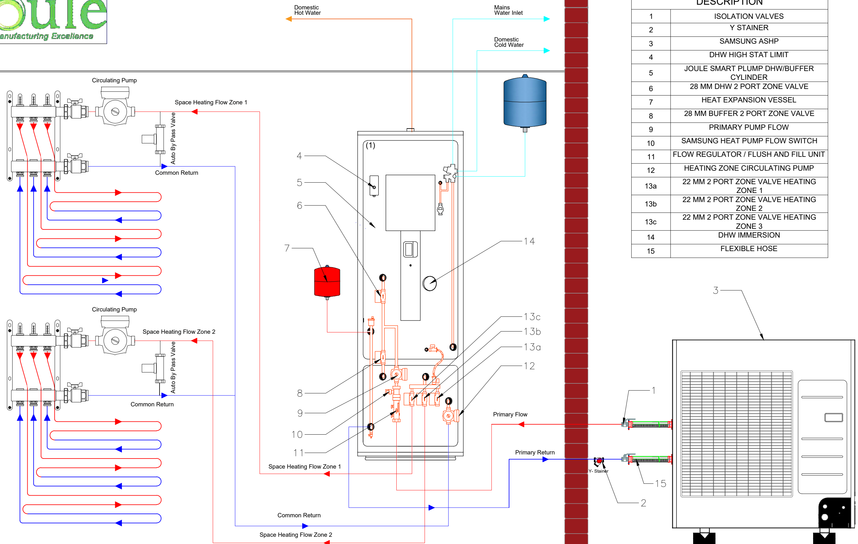
SAMSUNG ASHP WITH SMARTPLUMB DHW WITH 2 HEATING ZONE 2XUFHs
