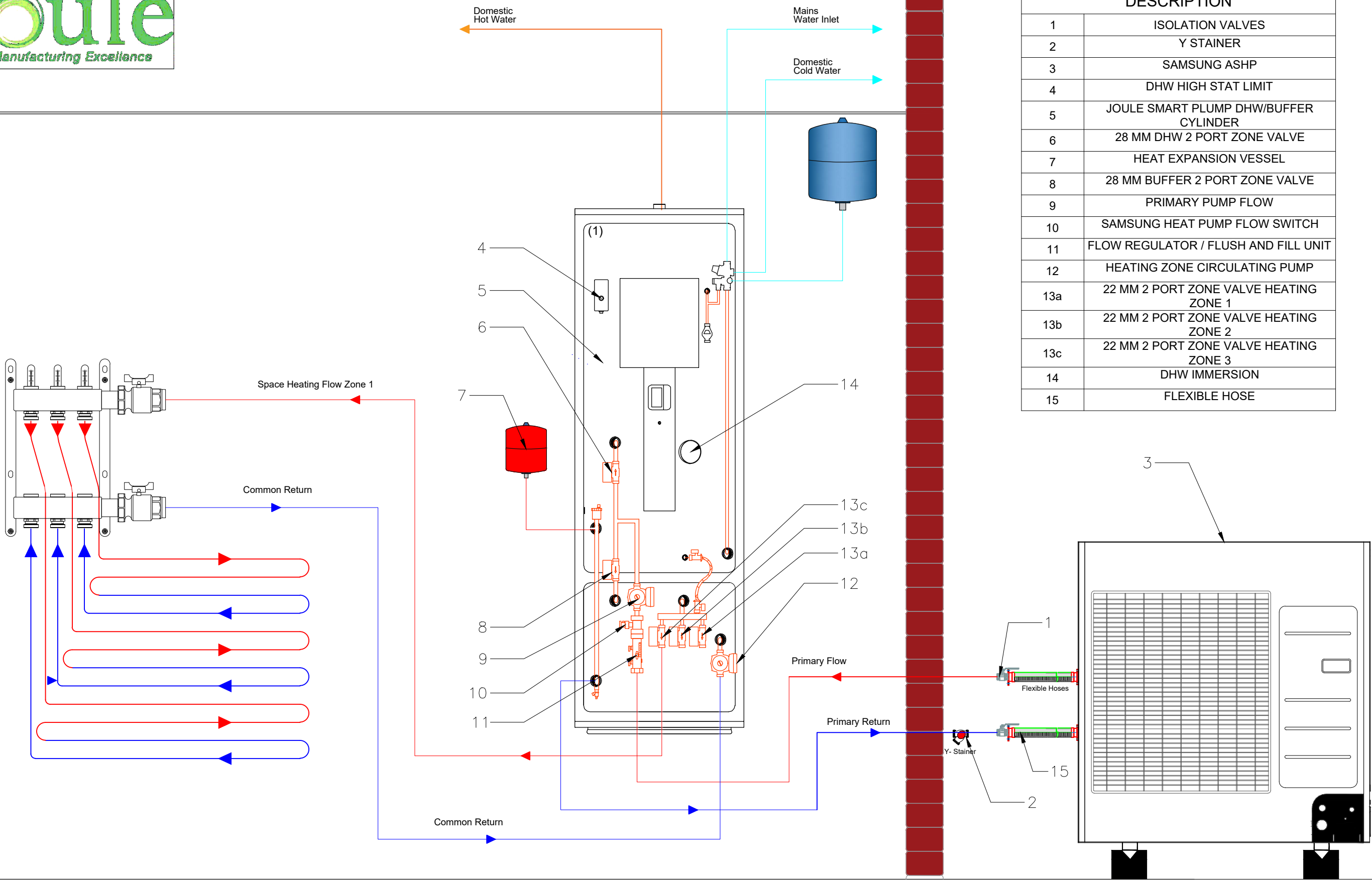
SAMSUNG ASHP WITH SMARTPLUMB DHW WITH 1 HEATING ZONE 1XUFH Front View of Unit & Cylinder
