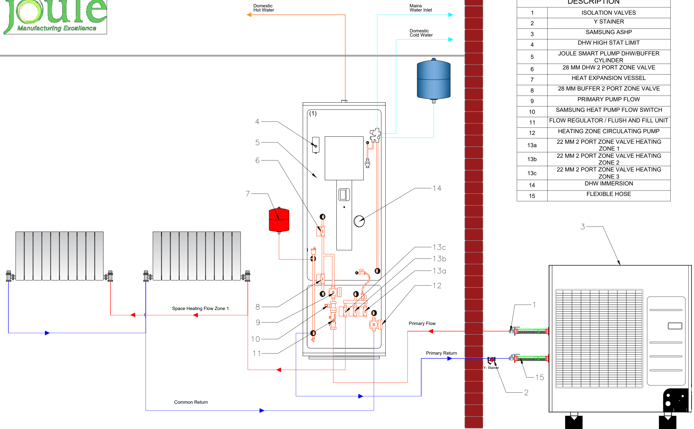
SAMSUNG ASHP WITH SMARTPLUMB DHW WITH 1 HEATING ZONE 1XRADs Front View of Unit & Cylinder
