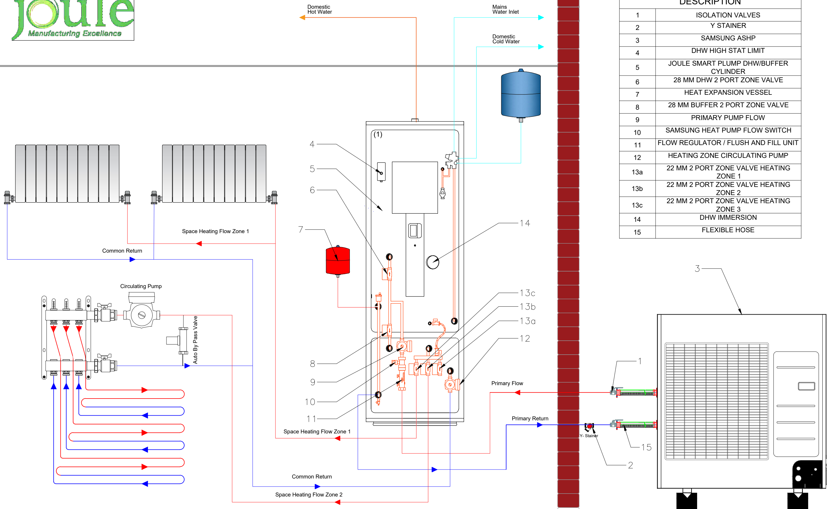
SAMSUNG ASHP WITH SMARTPLUMB DHW WITH 2 HEATING ZONE 1XRADs & 1XUFHs
